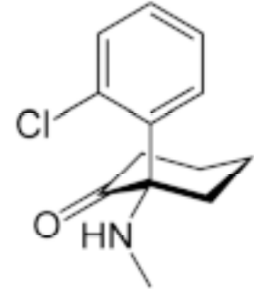
Figure 1: The structure of ketamine
